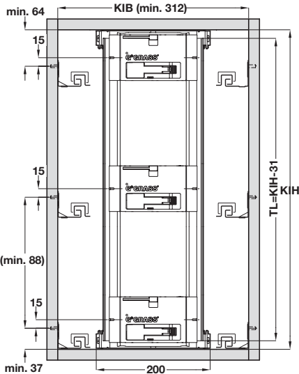
Position of opening unit Dynapro
