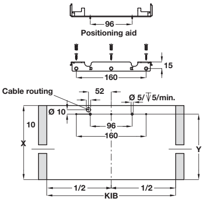
Fixing brackets top/bottom
