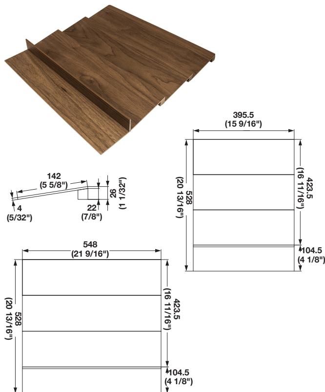
→ Stepped Spice Holders
