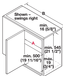
A = Clear opening dimension
