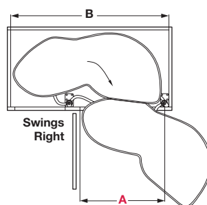
A = Clear opening dimension
