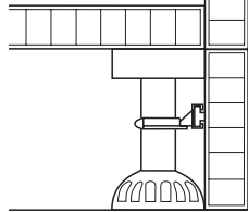
Mounting with the toe kick panel clip
