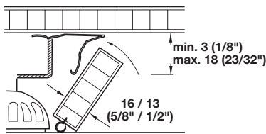
Mounting with the toe kick panel spring - front toe kick
