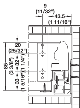
Rear panel installation dimensions
