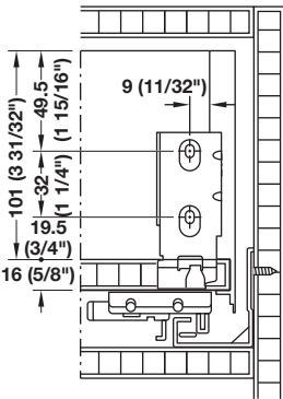
Rear panel installation dimensions
