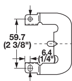
Front clip-on bracket
