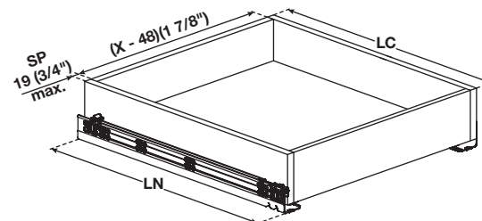
Drawer dimensions and drilling Full extension runner for 19 mm (3/4") drawer material
