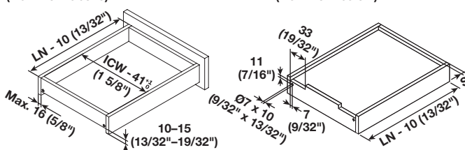
Drawer with front (view from above)
