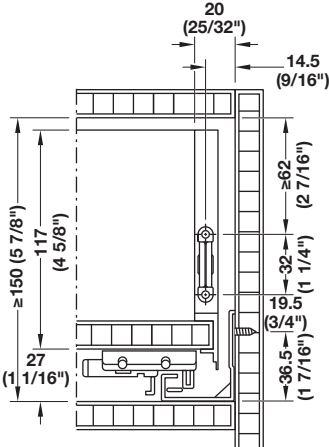
Internal installation height
