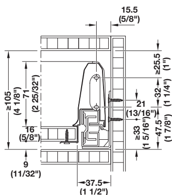
Internal installation height
