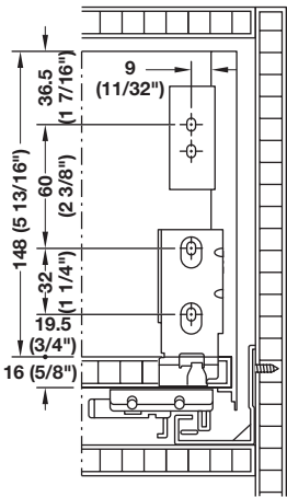
Rear panel installation dimensions
