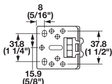
Rear metal bracket
